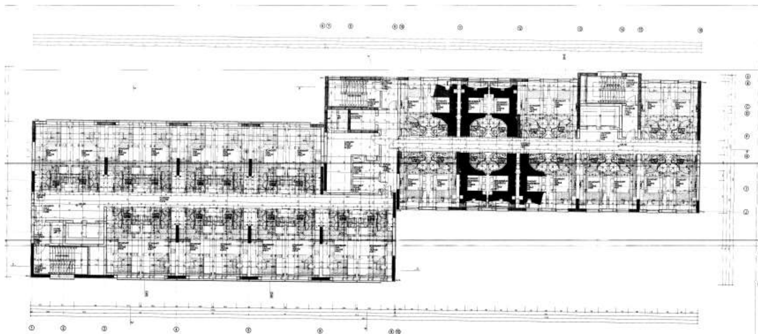
6. KAT PLANI 1/100
